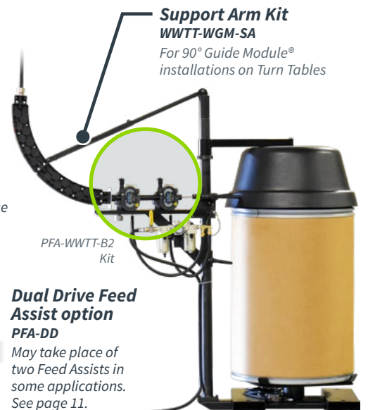
Wire Pilot® Turn Table Adapter Kit with Dual Feed Assists and Large Wire Wizard® Guide Modules Ideal setup for many SAW applications
